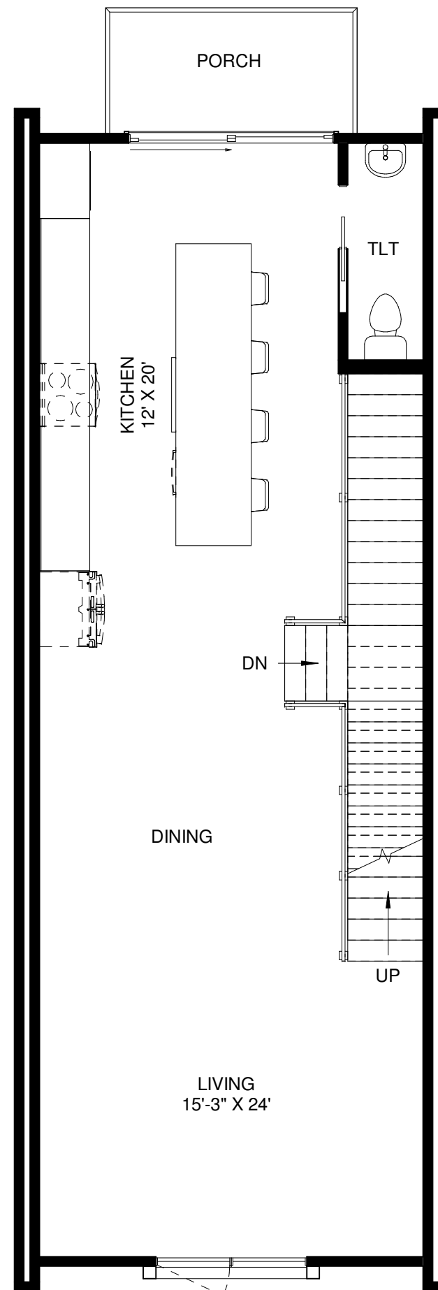
SECOND FLOOR
