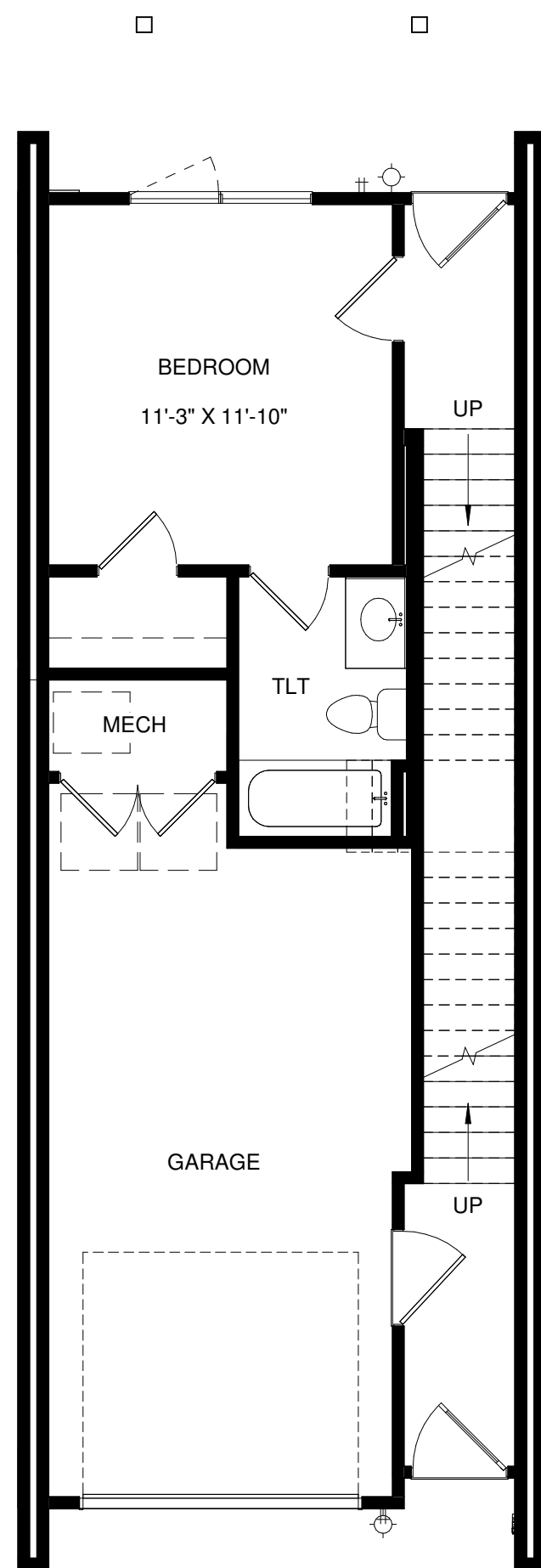
FIRST FLOOR
