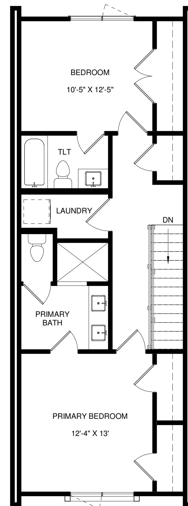
THIRD FLOOR
